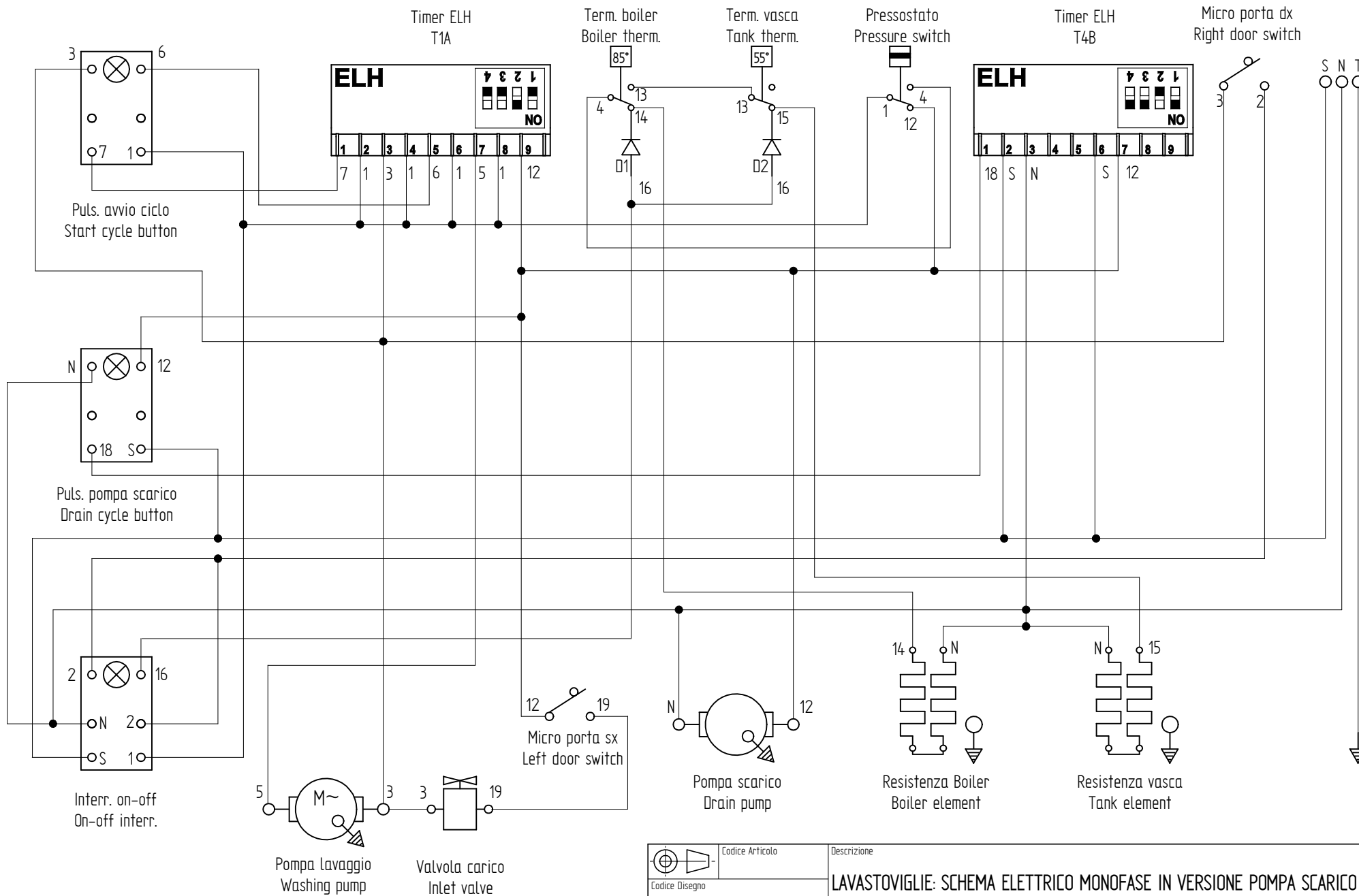
DISHWASHERS: ELECTRICAL WIRING SINGLEPHASE SCHEME WITH BUILT-IN DRAIN PUMP
